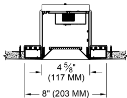
4U - FOUR SIDED ULTRIM FRAME
