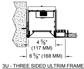
3U - THREE SIDED ULTRIM FRAME
