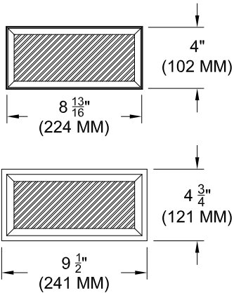
REFLECTED PLAN VIEW
