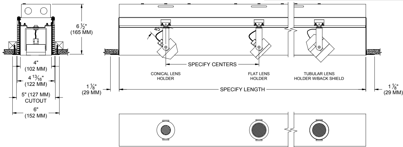
REFLECTED PLAN VIEW
