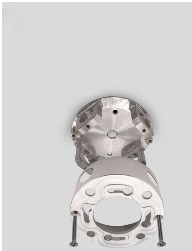
Step 3- Attach surface mounted j-box to ceiling plate with #8-32 counter sink screws (supplied by SLI)
