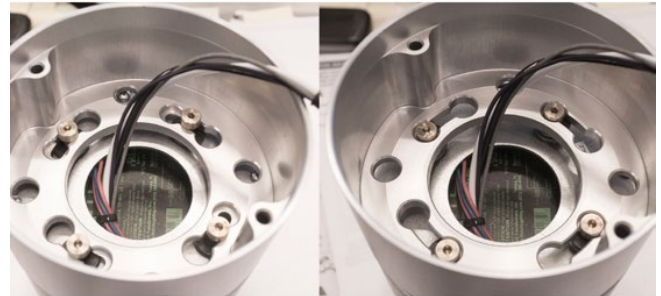
Step 6- Twist & Lock Clockwise. Gold pins must lock into keyway slot. Test power.
