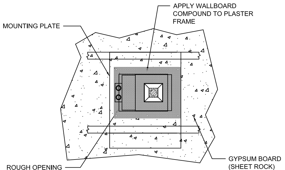
REFLECTED PLAN VIEW
