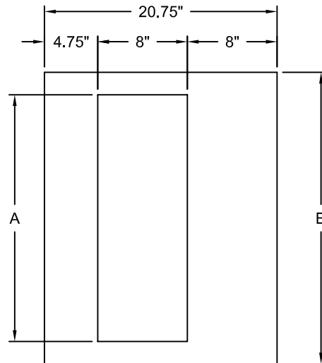
MOUNTING PLATE 16 GA. GALVANIZED STEEL
